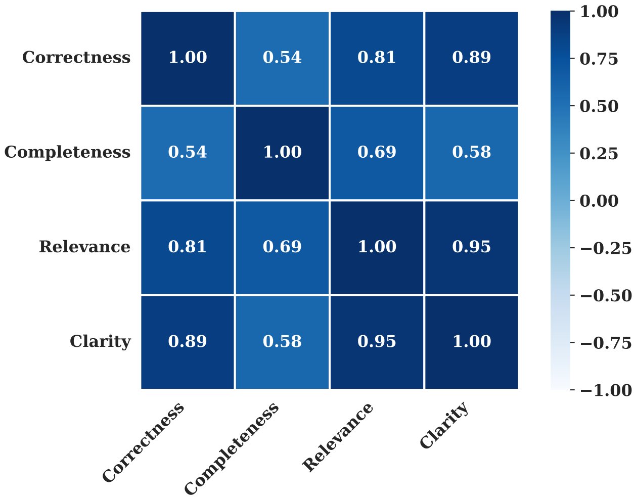
Correlation Matrix: RAG Chatbot Metrics (Aggregated across all Questions)
